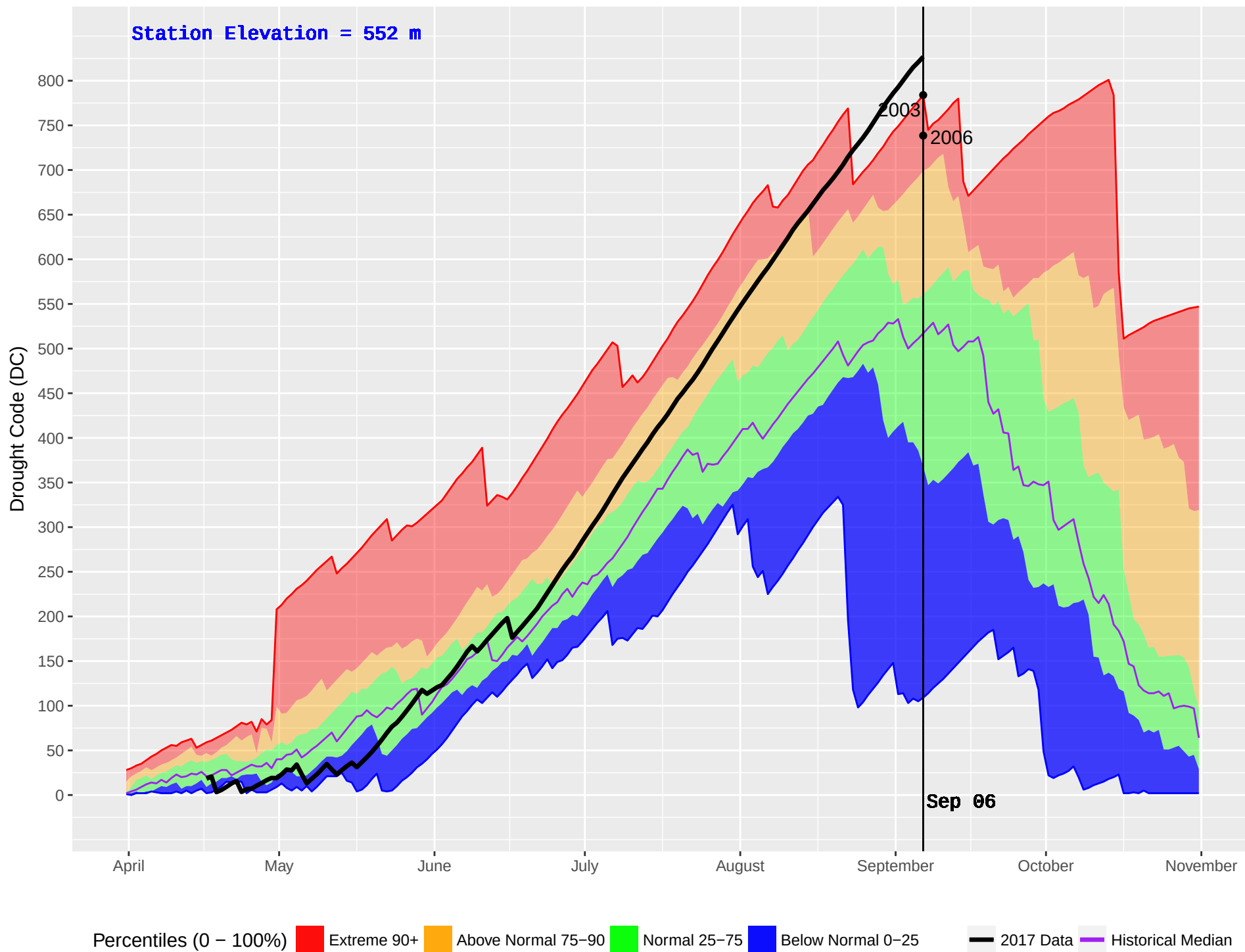
NAHATLATCH (316) : Historical (2001–2016) and Current (2017) Noon Drought Code (DC)
