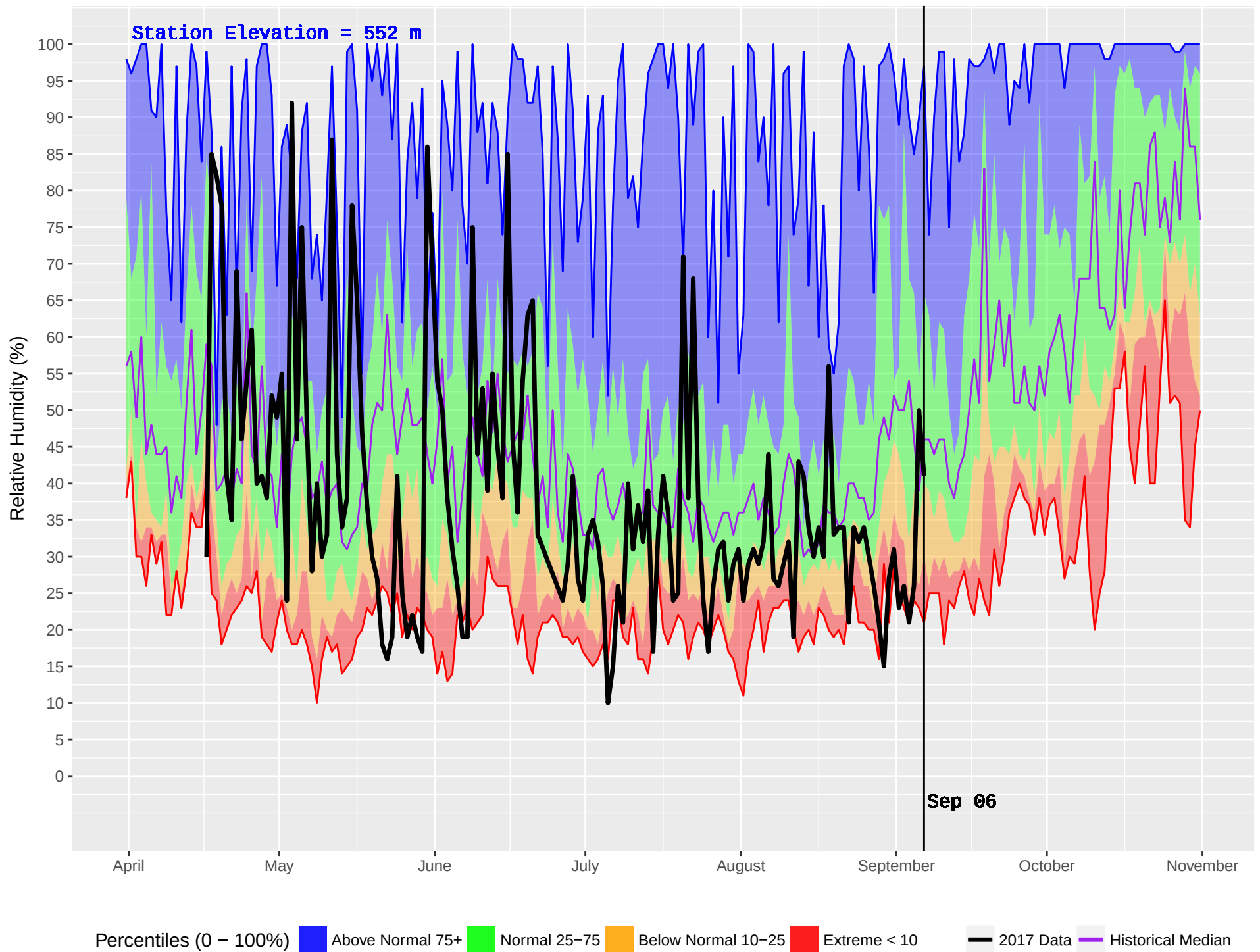
NAHATLATCH (316) : Historical (2001–2016) and Current (2017) Noon Relative Humidity
