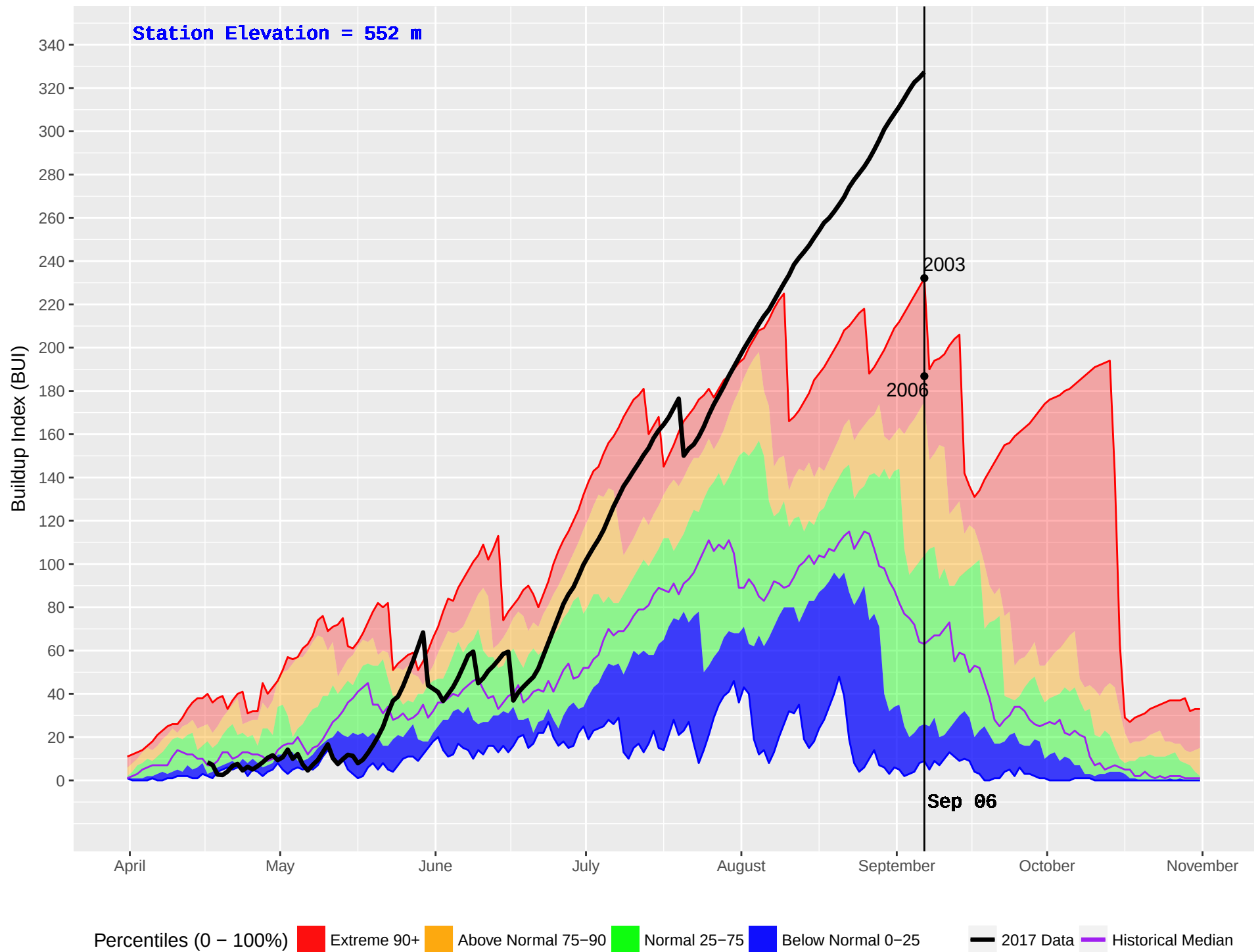
NAHATLATCH (316) : Historical (2001–2016) and Current (2017) Noon Buildup Index (BUI)
